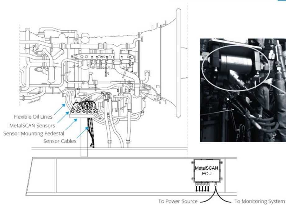
MetalSCAN Installation into Scavenge Lines on GE LMS100 Engine
